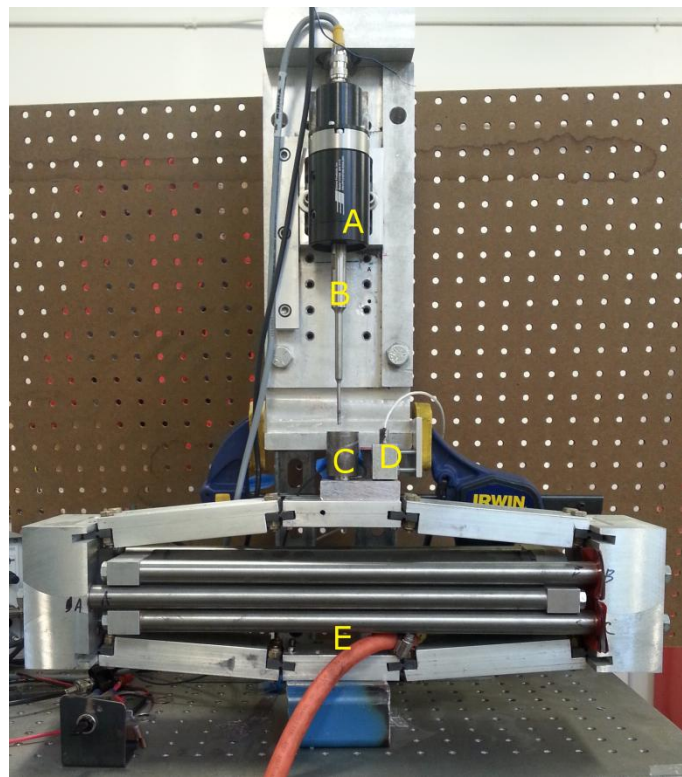
Figure 33 Experimental setup, comprised of CU-18 vibration transducer (A), titanium horn (B), lower die (C), displacement sensor (D), bulk motion transducer (E)
