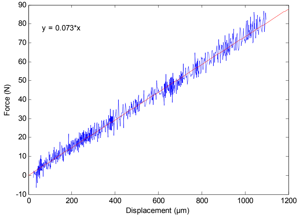
Figure 19 Manual testing used to determine effective bending spring rate of flexures. Force required to move lever system at its output was measured as a function of displacement, also measured at the output.
