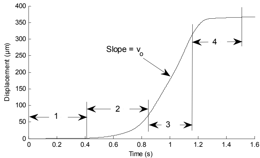
Figure 34 Phases of welding demonstrated on a welding sample of 0.5 mm thick ABS welded to 358 µm at 234 N
