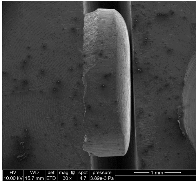
Figure 30 SEM view of punched surface, showing fractured and burnished areas.
